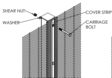
DETAIL ASSEMBLY INTERMEDIATE POST
