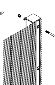
DETAIL ASSEMBLY END/START POST
