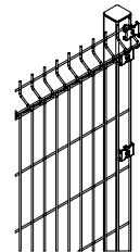
DETAIL ASSEMBLY END/START POST
