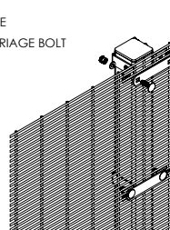
DETAIL ASSEMBLY END/START POST
