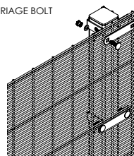
DETAIL ASSEMBLY END/START POST
