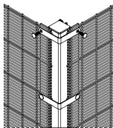
DETAIL ASSEMBLY CORNER POST
