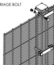
DETAIL ASSEMBLY END/START POST
