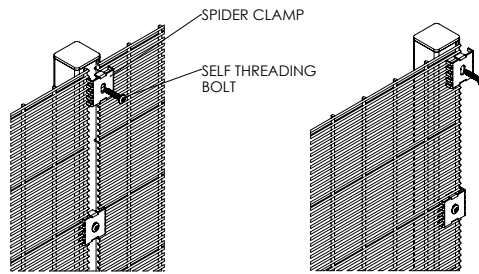
DETAIL ASSEMBLY INTERMEDIATE POST
