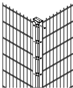
DETAIL ASSEMBLY CORNER POST
