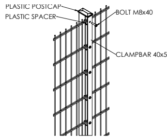
DETAIL ASSEMBLY INTERMEDIATE POST
